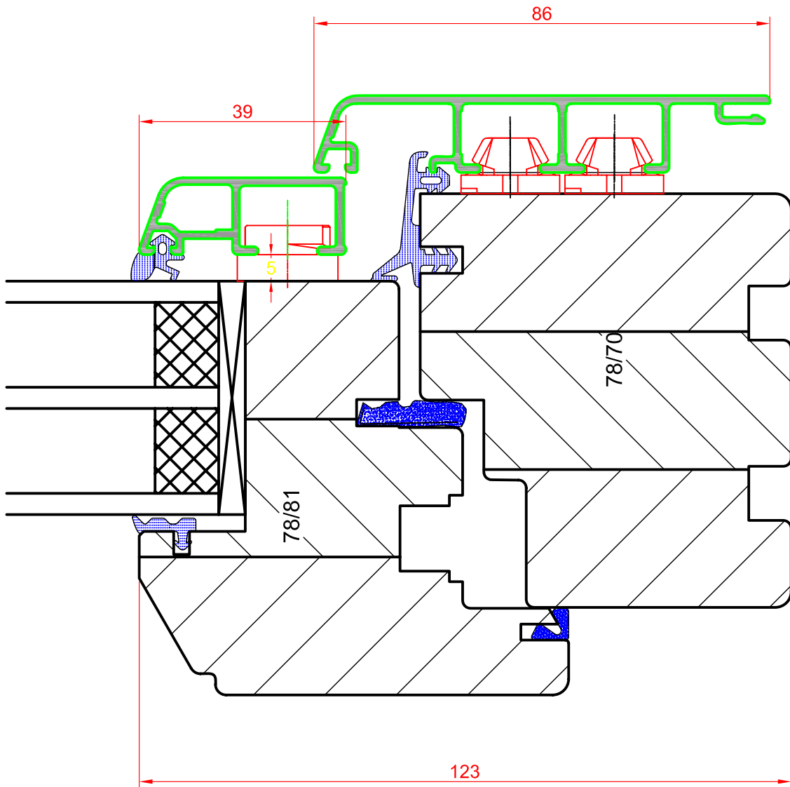
WINDOW SIDE FRAME & SASH JUNCTION - SECTION
