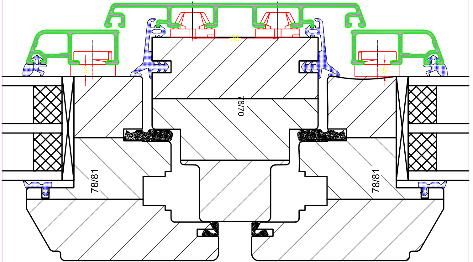
SECTION THROUGH WINDOWS WITH VERTICAL POST
