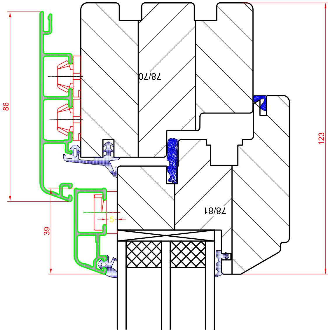
WINDOW AND FRAME SECTION FROM ABOVE
