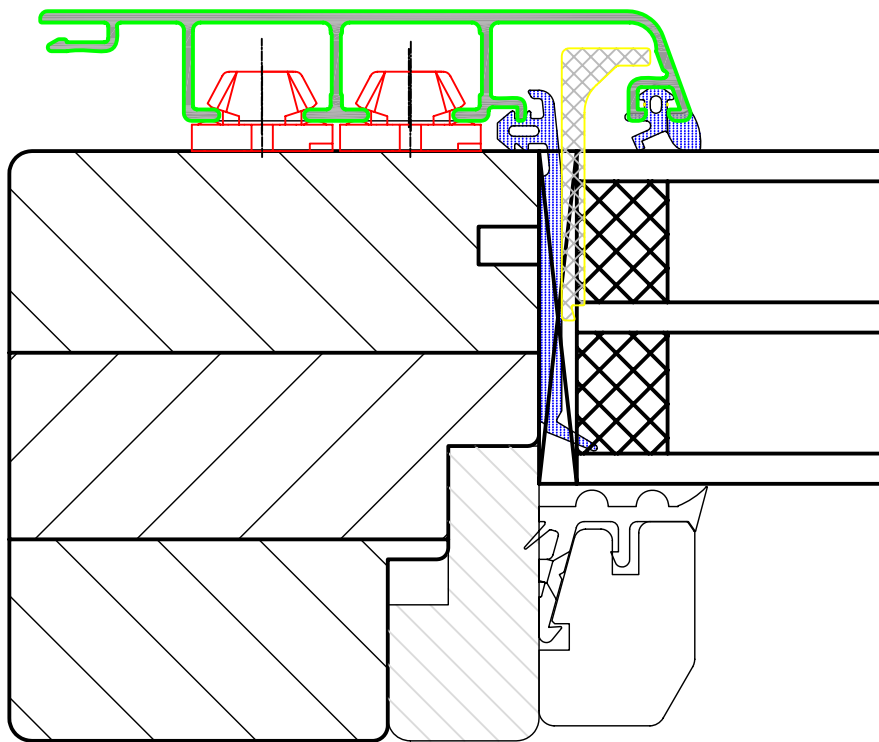
TOP AND SIDE WINDOWS FIXED GLAZING
