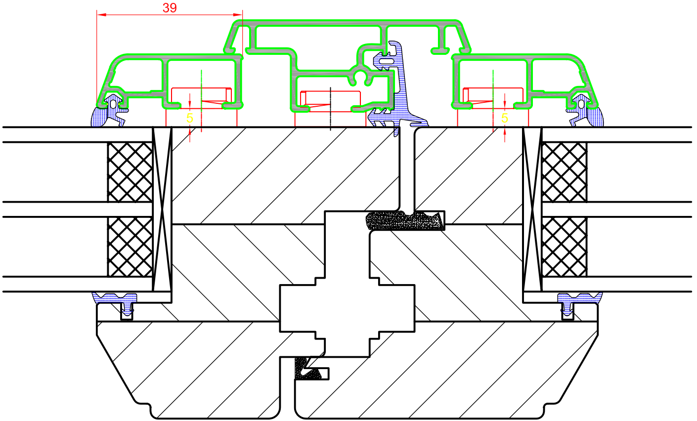
FIXED WINDOW AND OPENING WINDOW SECTION
