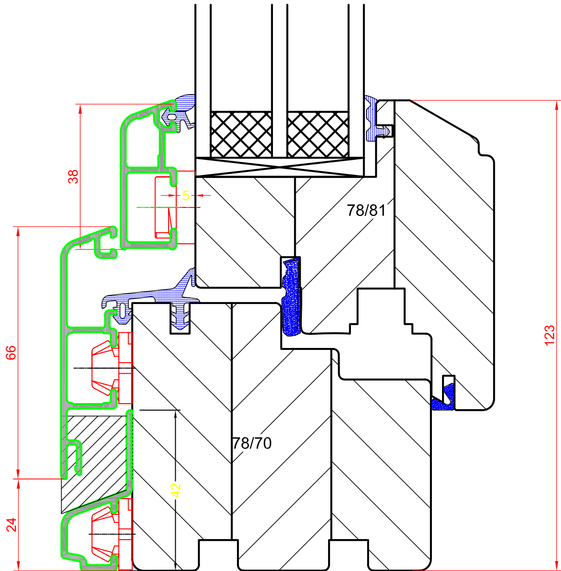
WINDOW FRAME BASE WITH OPENING LIGHT ABOVE SUITABLE FOR STONE CILL BELOW
