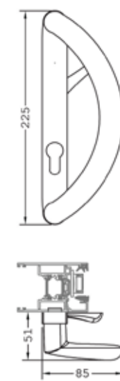
D-shaped handle (colour coded)
