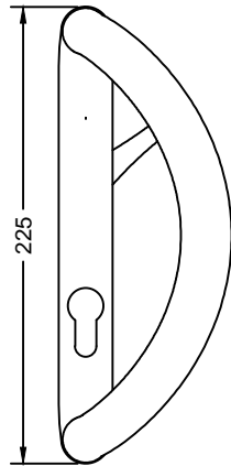
'D' Shaped Handle With Keylock
